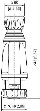
8572/14 SolConeX coupling
