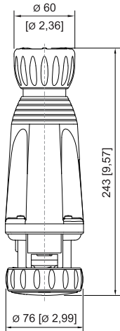
8572/14 SolConeX Kupplung
