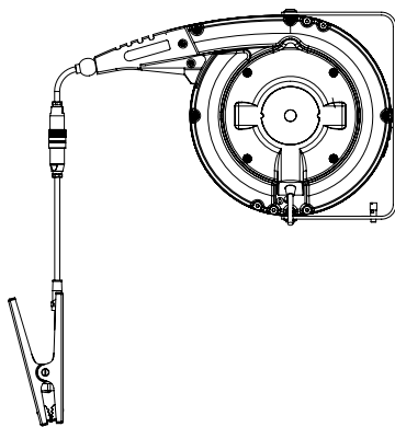
Fig. 24: Self retracting reel 601KR/AW in aluminium with ground clamp 70BGS04
