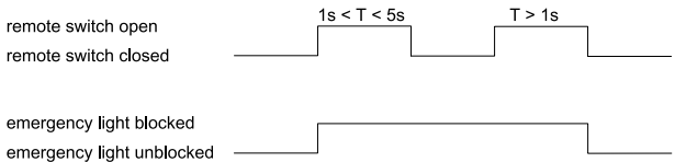
Logic 2
