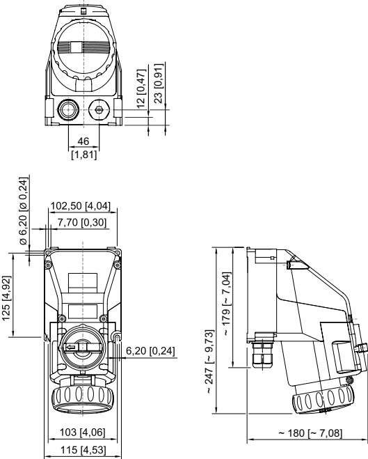
Wandsteckdose 4-polig / 5-polig
