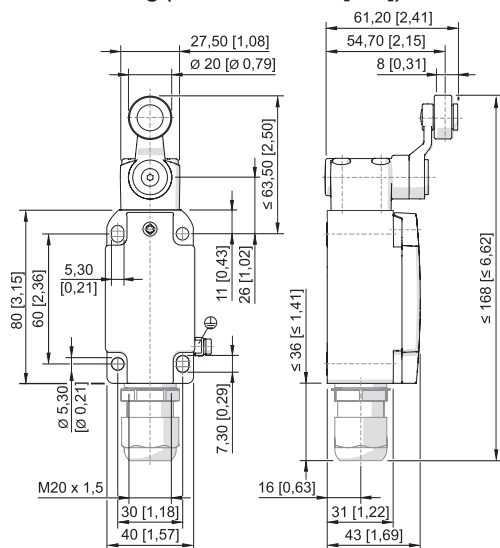
Schwenkhebel 8074/2-1-D-40
