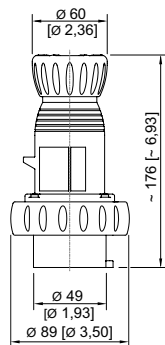
Stecker 4-polig
