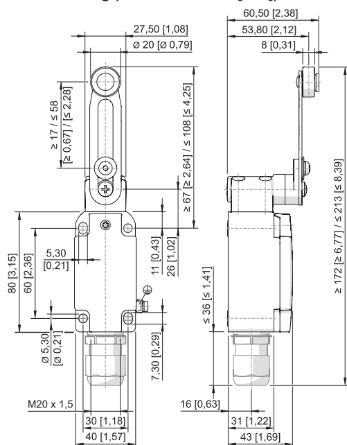
Schwenkhebel 8074/2-4-DS-40
