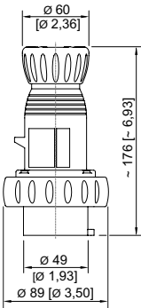
Stecker 4-polig
