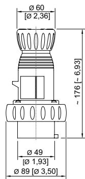
Stecker 4-polig
