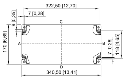
8146/.06. 8146/.061: h = 91 mm [3.58 in] 8146/.062: h = 131 mm [5.16 in]
