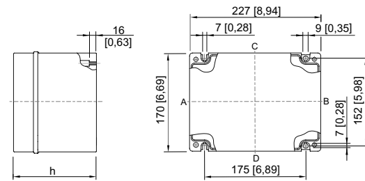
8146/.06. 8146/.061: h = 91 mm [3.58 in] 8146/.062: h = 131 mm [5.16 in]
