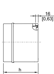
8146/S7. 8146/S71: h = 91 mm [3.58 in] 8146/S73: h = 150 mm [5.91 in]
