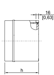
8146/.05. 8146/.051: h = 91 mm [3.58 in] 8146/.052: h = 131 mm [5.16 in]
