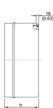
8146/.08. 8146/.081: h = 91 mm [3.58 in] 8146/.082: h = 131 mm [5.16 in] 8146/.083: h = 150 mm [5.91 in] 8146/.084: h = 171 mm [6.73 in] 8146/.085: h = 190 mm [7.48 in] 8146/.086: h = 230 mm [9.06 in]
