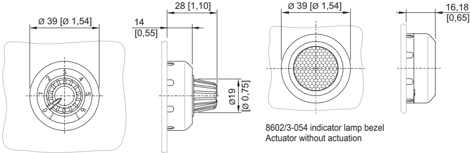
8602/3-092 potentiometer bezel Actuator with radial actuation
