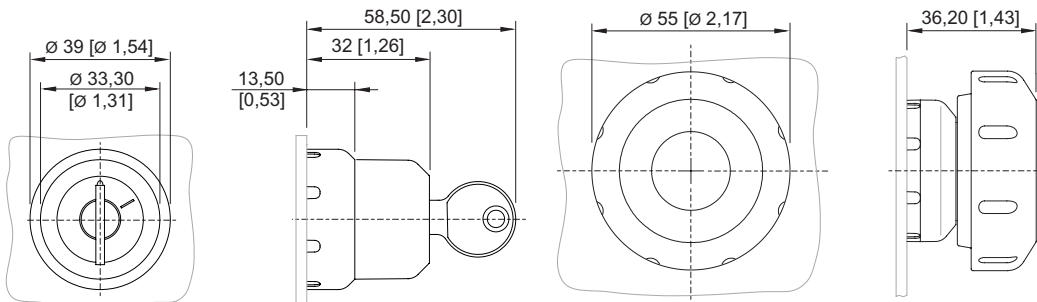
8602/3-014 red/black mushroom pushbutton 8602/3-703 black/black mushroom pushbutton Actuator with axial actuation
