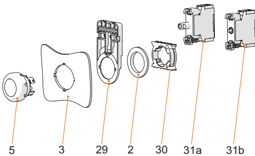
Front installation mounting with Series 8010/6 indicator lamp and Series 8082/3 contact element
