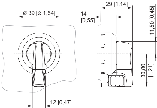
8602/3-727 axial rotary actuator, lockable Actuator with axial actuation
