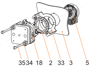
Front installation mounting with Series 8008 control switch
