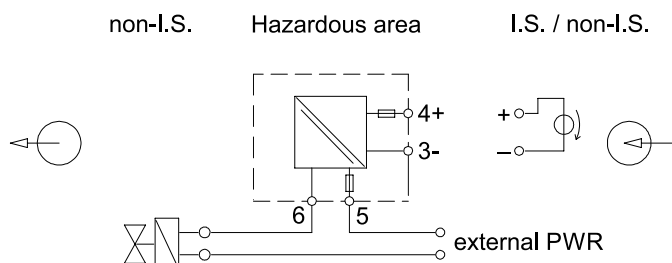
Connection diagram 9174/12
