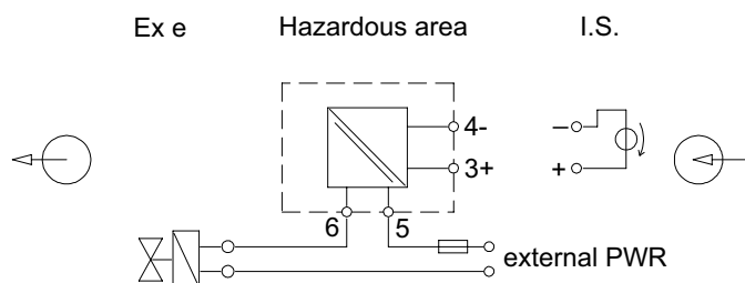
Connection diagram 9174/10
