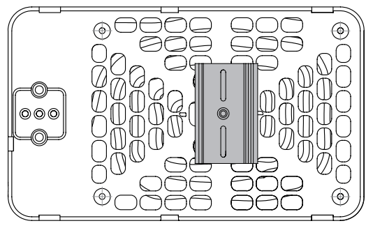
Optional DIN rail module, placed in vertical position
