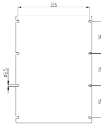
TEF 4500 901 MOUNTING DIMENSIONS
