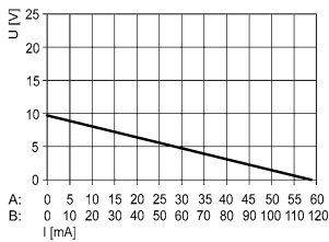
9175/0-12-11, 9176/0-12-00 output characteristic
