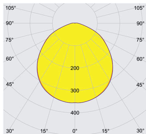
Without internal reflector, protection glass diffuse
