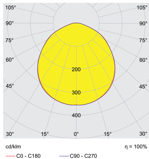
Without internal reflector, protection glass diffuse
