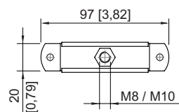
Luminaire with mounting bracket for a thread
