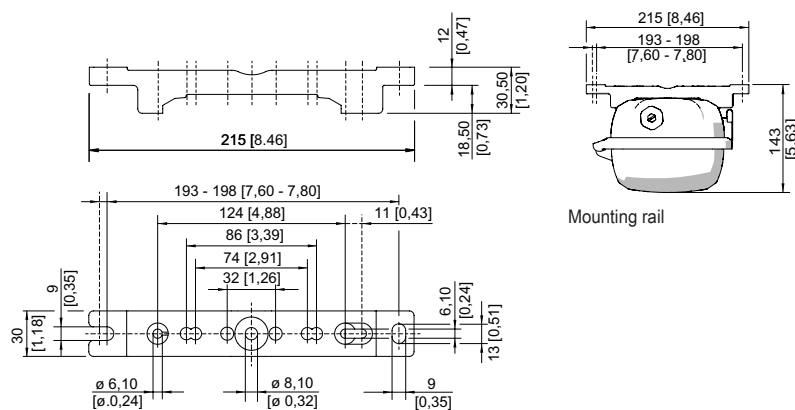
Mounting rail
