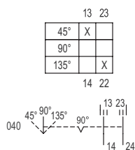
Switching arrangement 8008/-040
