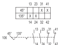
Switching arrangement 8008/-106
