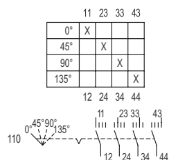
Switching arrangement 8008/-110
