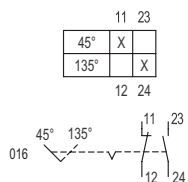
Switching arrangement 8008/-016
