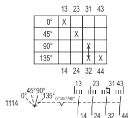
Switching arrangement 8008/-1114
