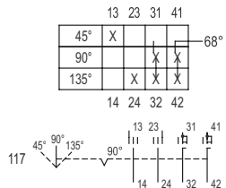
Switching arrangement 8008/-117
