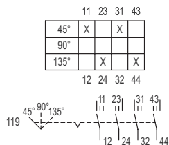
Switching arrangement 8008/-119
