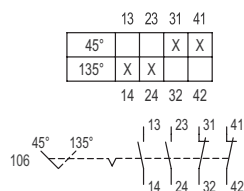
Switching arrangement 8008/-106
