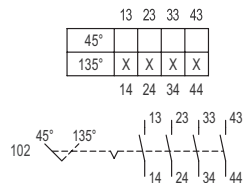
Switching arrangement 8008/-102
