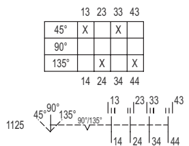
Switching arrangement 8008/-1125
