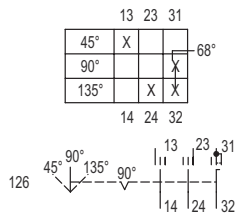
Switching arrangement 8008/-126
