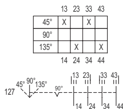
Switching arrangement 8008/-127
