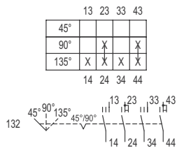
Switching arrangement 8008/2-132
