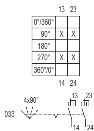
Switching arrangement 8008/-033
