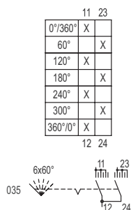
Switching arrangement 8008/-035
