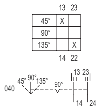
Switching arrangement 8008/-040
