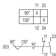
Switching arrangement 8008/-053
