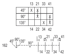
Switching arrangement 8008/-162
