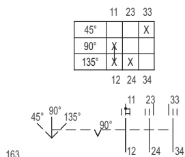
Switching arrangement 8008/-163
