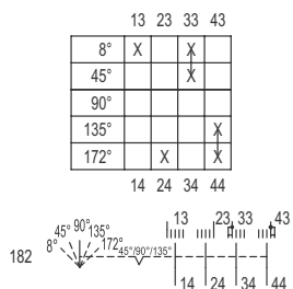
Switching arrangement 8008/-182
