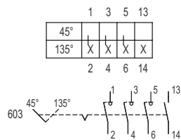
Switching arrangement 8008/-603
