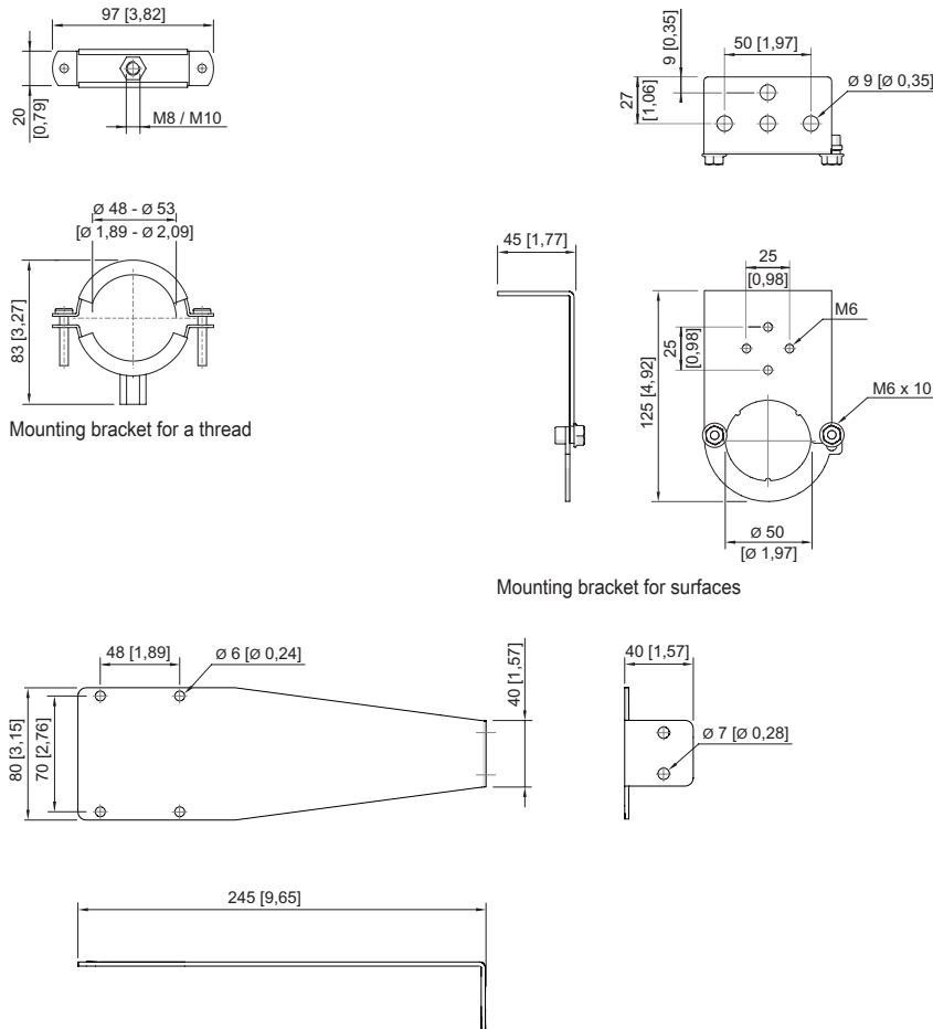
Mounting plate
