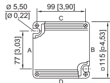
8118/2. Enclosure SZ 2
