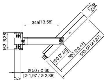
Floodlight with pole mounting
