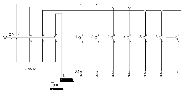
Circuit diagram 8146/5-ExV-...1P-T
