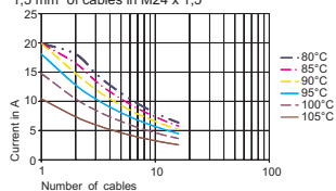
Current loading of 1,5 mm 2 of cables in M24 x 1,5
