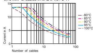
Current loading of 0,75 mm 2 of cables in M42 x 1,5 / ø 41
