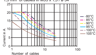
Current loading of 1,5 mm 2 of cables in M33 x 1,5 / ø 34
