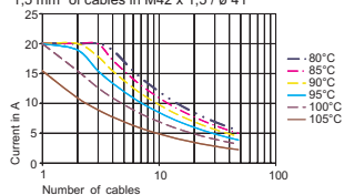
Current loading of 1,5 mm 2 of cables in M42 x 1,5 / ø 41
