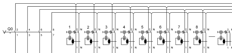
Circuit diagram 8146/5-ExV-...1N-D; 8264/5-ExV-...1N-D
