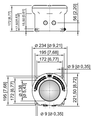
Enclosure size 3 with inspection window
